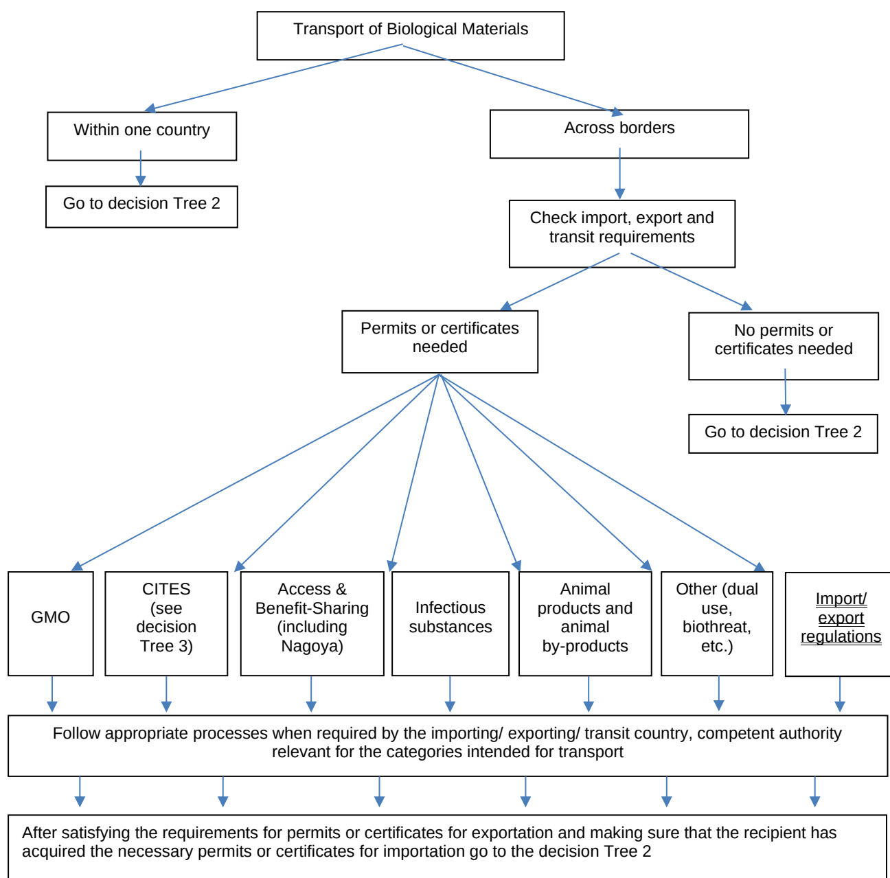
Decision Tree 1:
